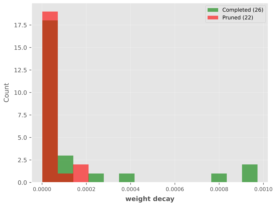
weight decay: Completed vs Pruned
